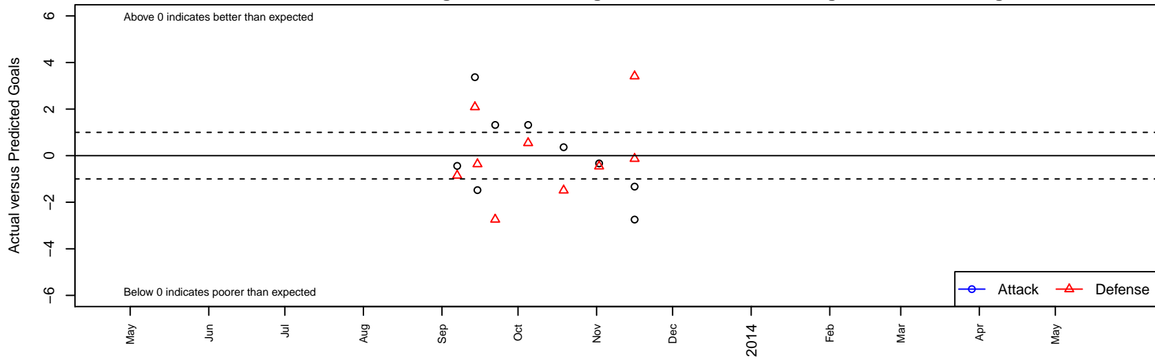
CWSA Grey G02 Dots are actual minus expected GF (blue circles) and GA (red triangles). Blue line is smoothed change in attack strength. Red is smoothed change in defense strength.
